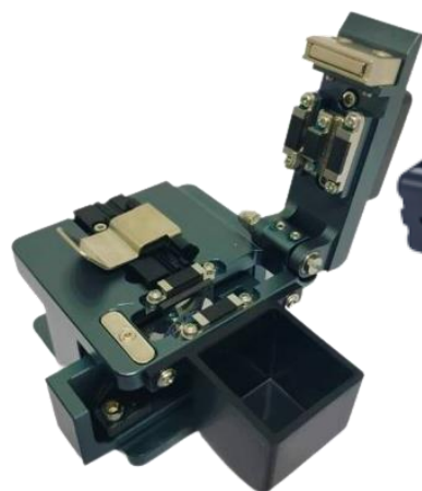
FIBER CLEAVER V320S HEAVY DUTY
